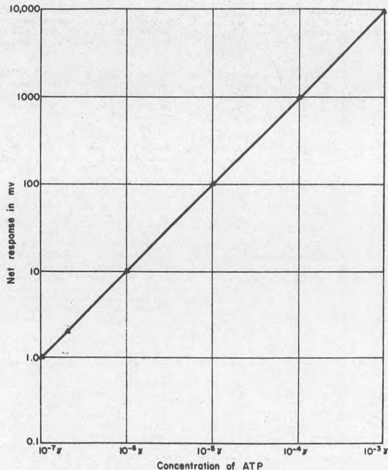
Figure 5 - Standard ATP curve on Bioluminescent detector.
