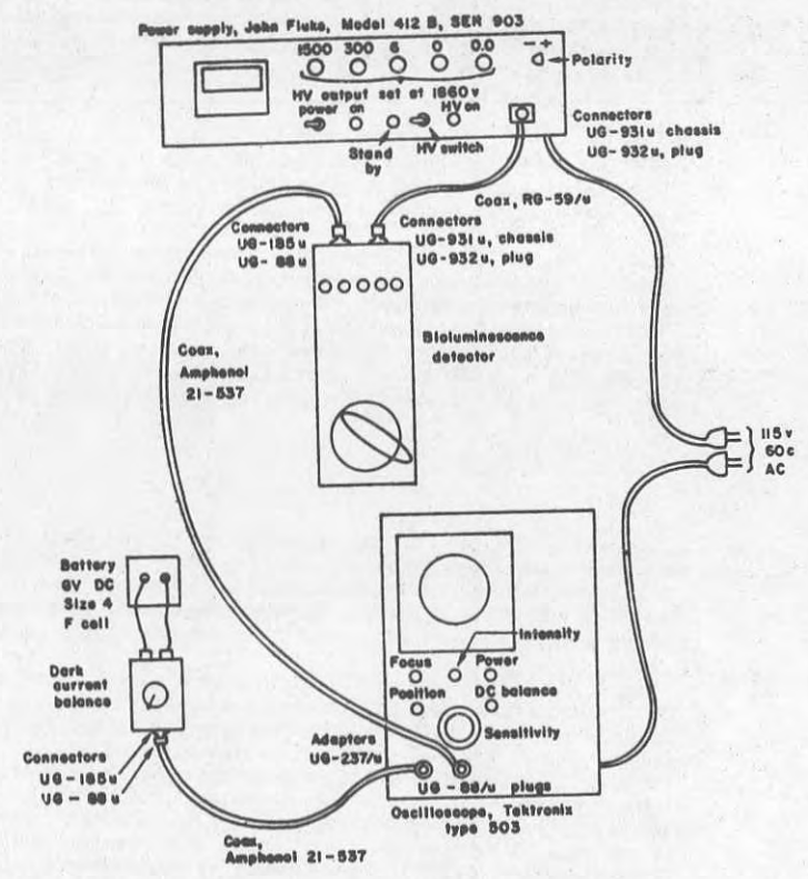
Figure 14 - Equipment connections and controls.
